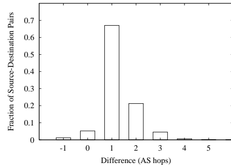
Fig. 3. Validating the shortest AS path model for routing policy.
