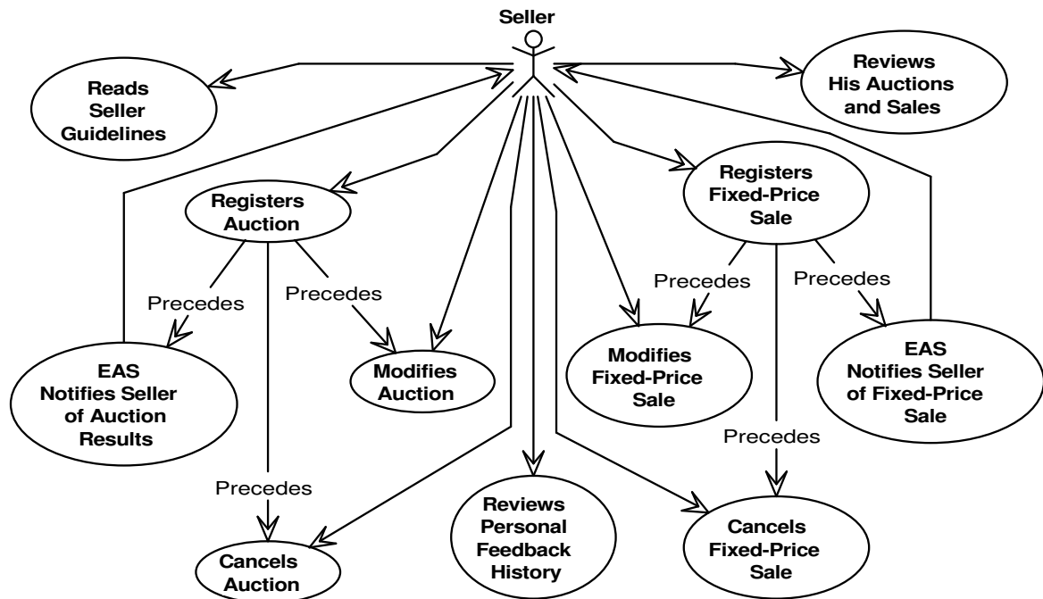
Figure 9: Seller Use Case Diagram
