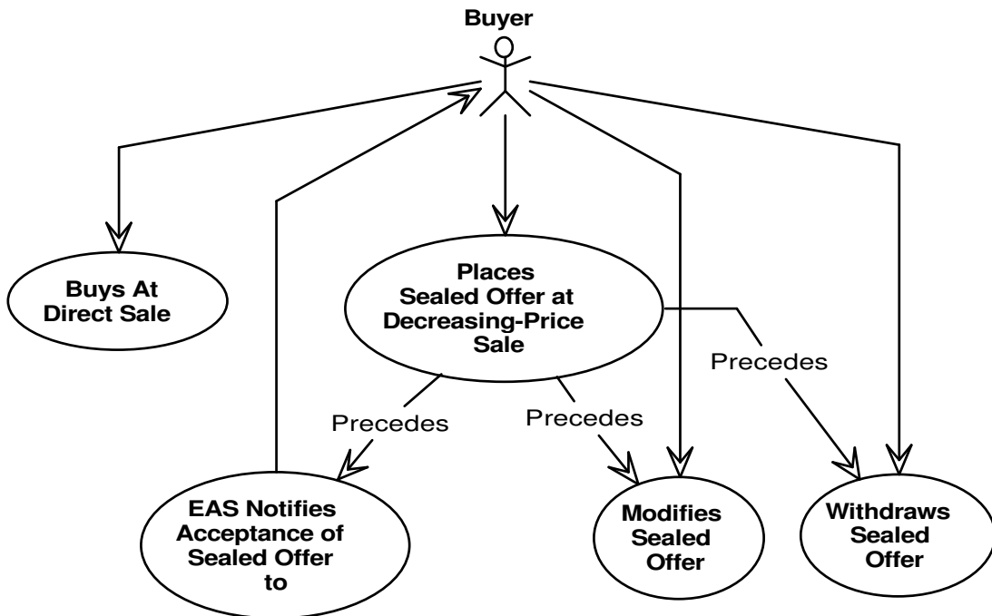
Figure 7: Direct Sale Buyer Use Case Diagram
