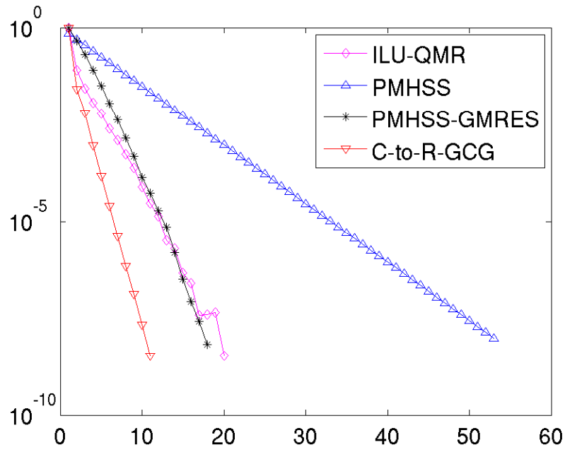
Figure 3: Problem 1: Convergence comparisons, FEM, problem size 16641, \omega = 1
