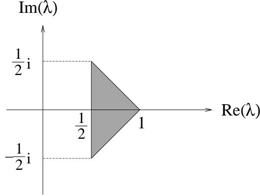
Figure 1: Eigenvalues of (A + B)^{-1}(A + iB)
