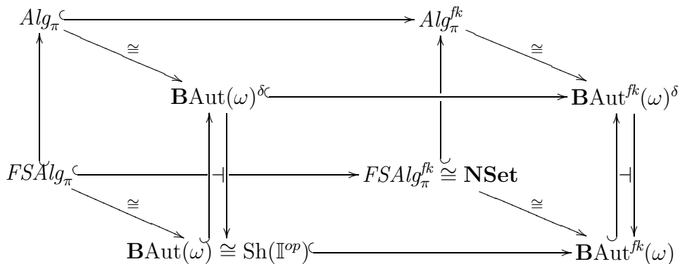
Fig. 2. The Permutation Algebra Cube, strengthened version.
